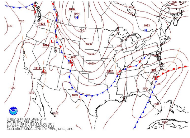
Figure 4: (a.) 500 hPa heights (dm), temperature ( ^{\circ}\text{C} ) and wind (kts) , and (b.) surface analysis from 09 UTC 26 February, 2015 (images courtesy of SPC and WPC).
