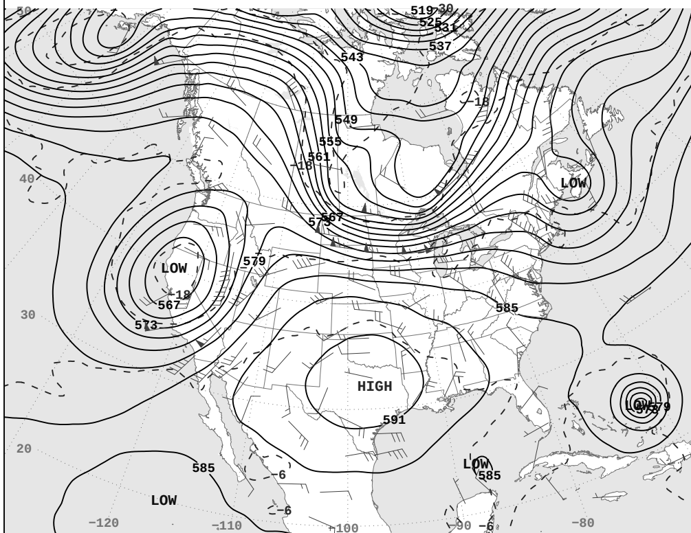
WED, SEP 21, 2022 500-Millibar Height Contours at 7:00 A.M. E.S.T.
