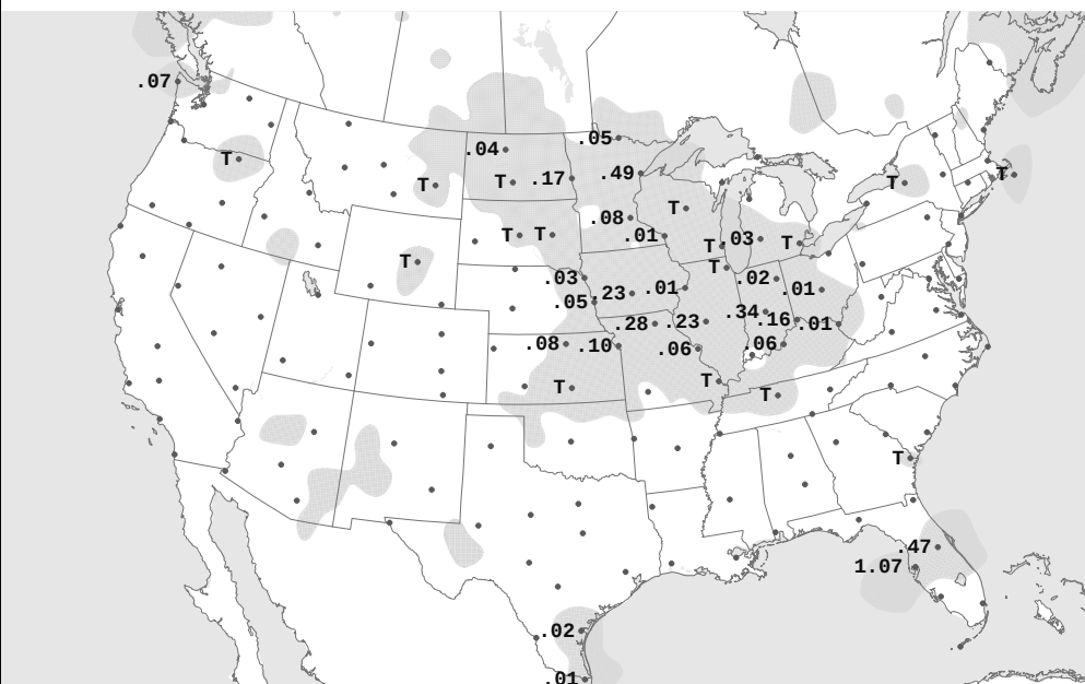
SAT, SEP 24, 2022 24-hour Precipitation Areas and Amounts Ending 7:00 A.M. E.S.T.
