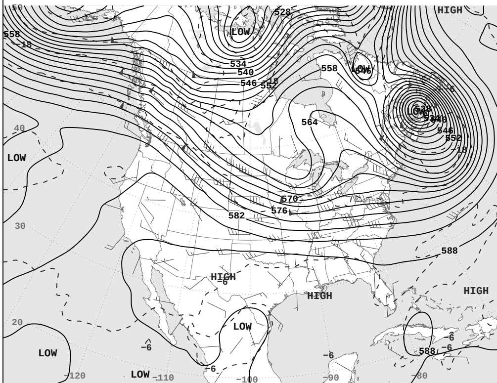
SAT, SEP 24, 2022 500-Millibar Height Contours at 7:00 A.M. E.S.T.
