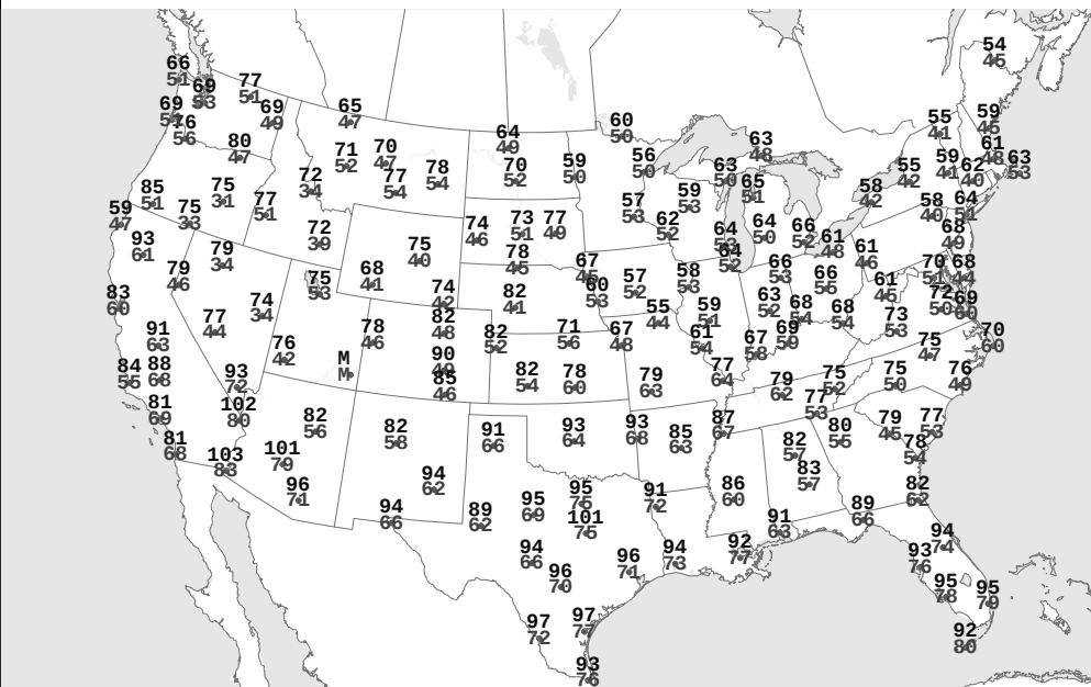
SAT, SEP 24, 2022 Highest and Lowest Temperature
