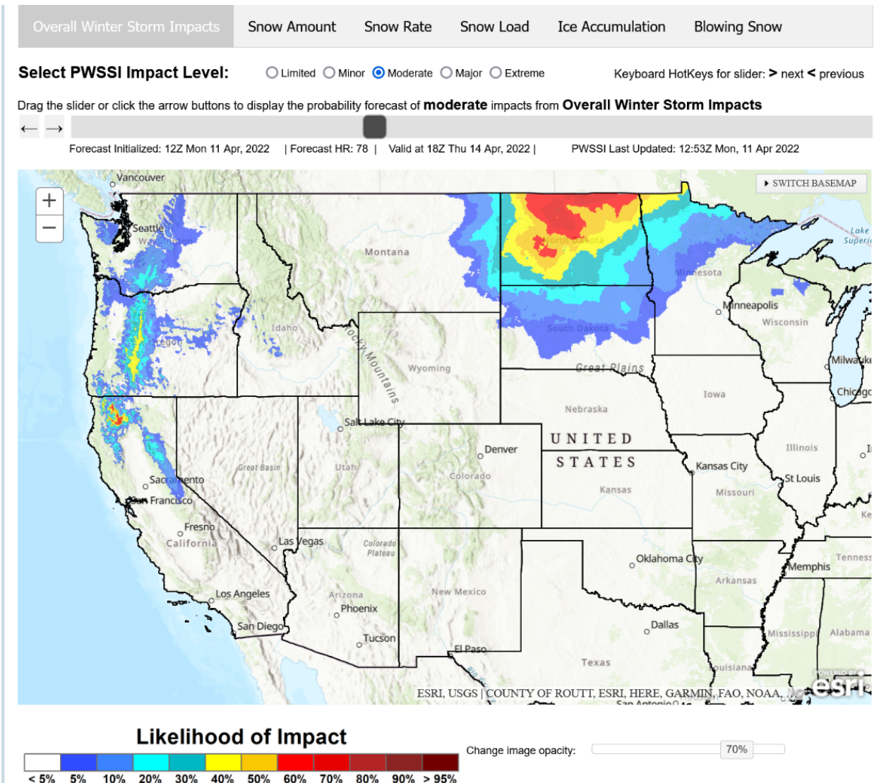
Figure B: Experimental Probabilistic Winter Storm Severity Index showing the likelihood of moderate Overall Winter Storm Impacts. Valid 18Z Thursday, April 14, 2022.
