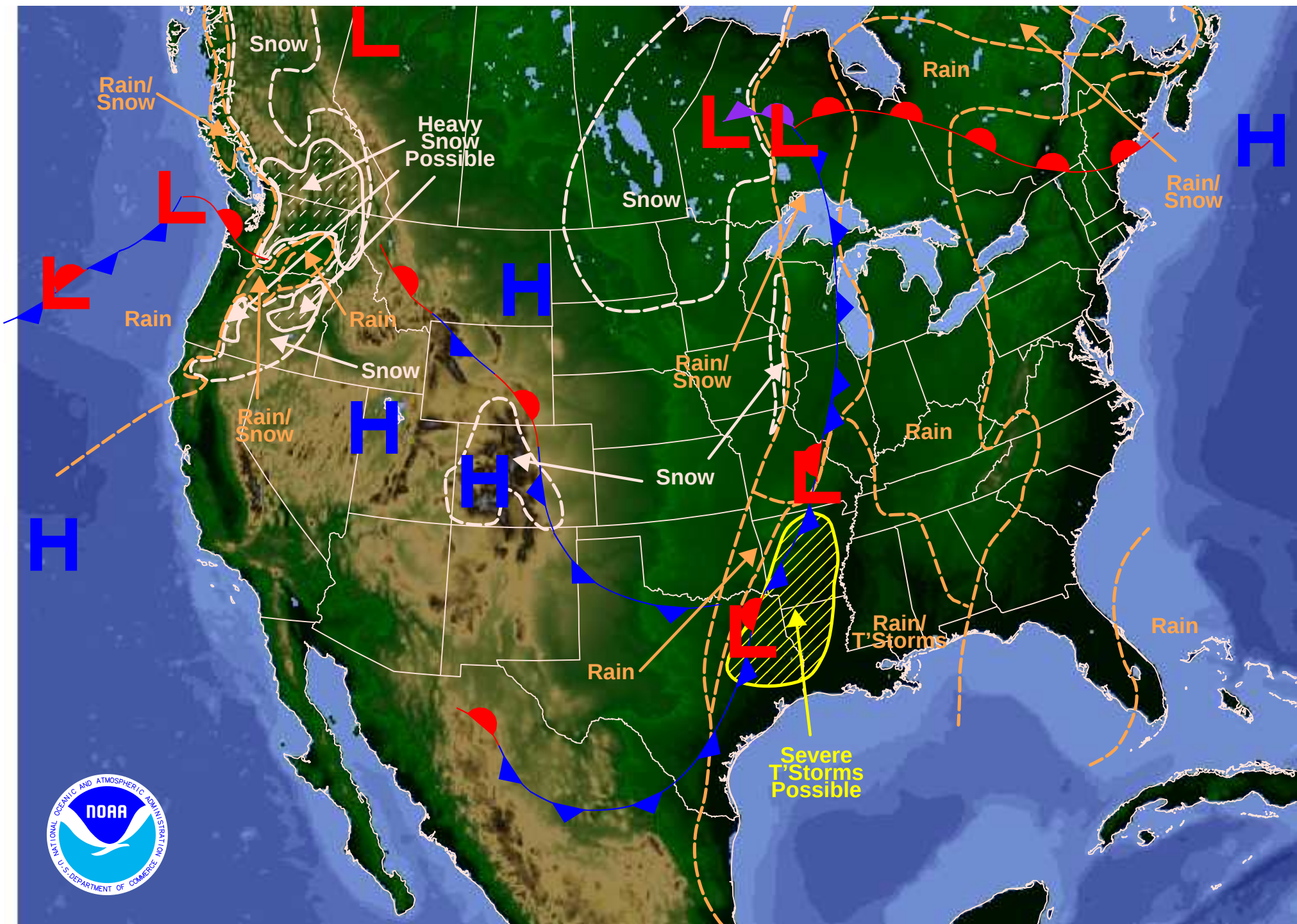
Weather Forecast for Sun, Nov 11, 2012, issued 3:41 PM EST DOC/NOAA/NWS/NCEP/Hydrometeorological Prediction Center Prepared by Ryan based on HPC, SPC, and NHC forecasts
