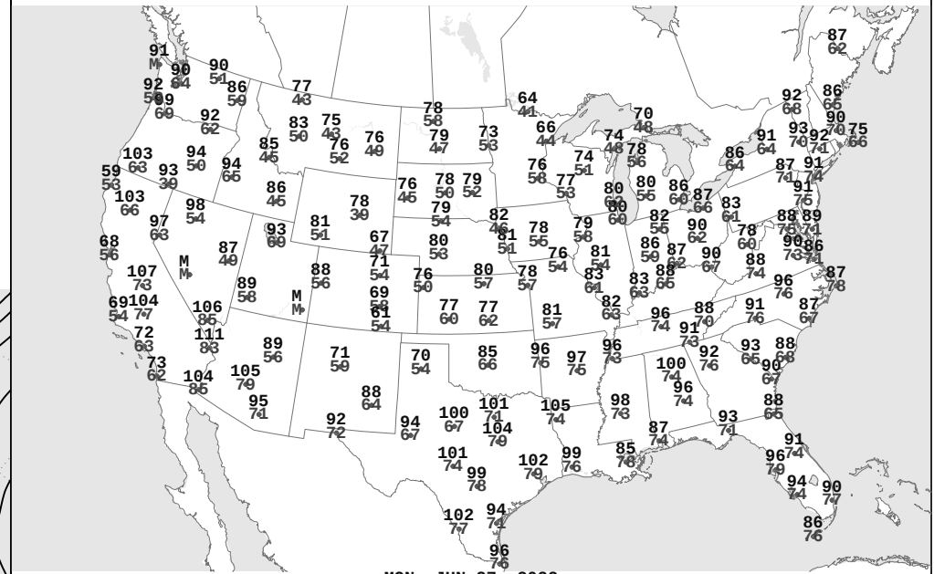
MON, JUN 27, 2022 Highest and Lowest Temperature
