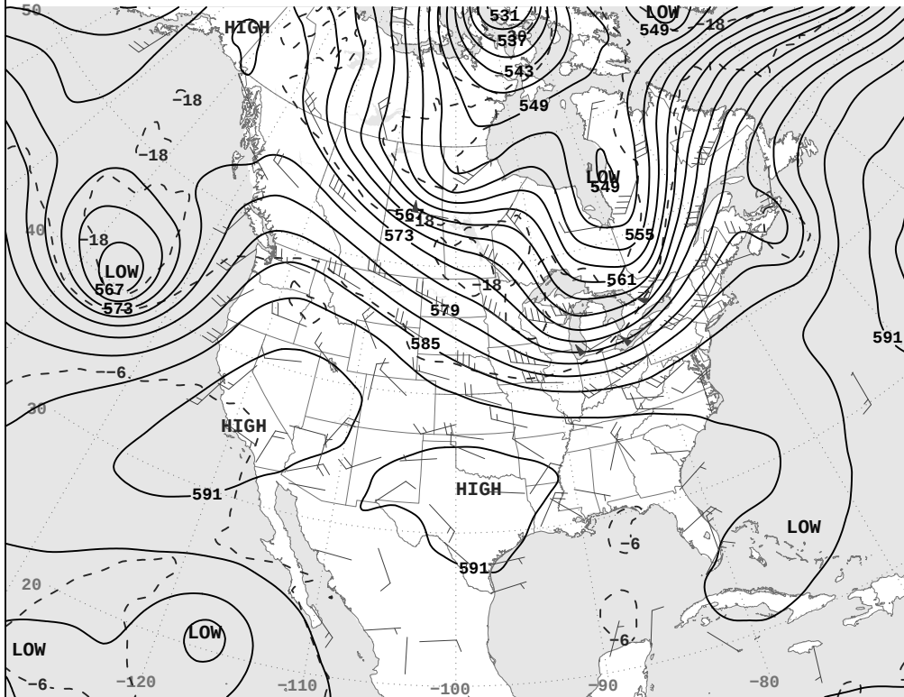
MON, JUN 27, 2022 500-Millibar Height Contours at 7:00 A.M. E.S.T.
