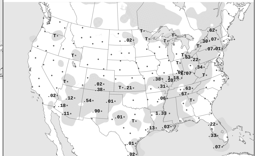
MON, JUN 27, 2022 24-hour Precipitation Areas and Amounts Ending 7:00 A.M. E.S.T.
