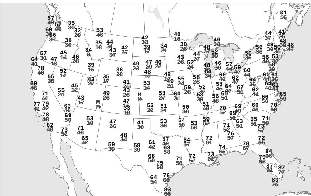
FRI, NOV 25, 2022 Highest and Lowest Temperature
