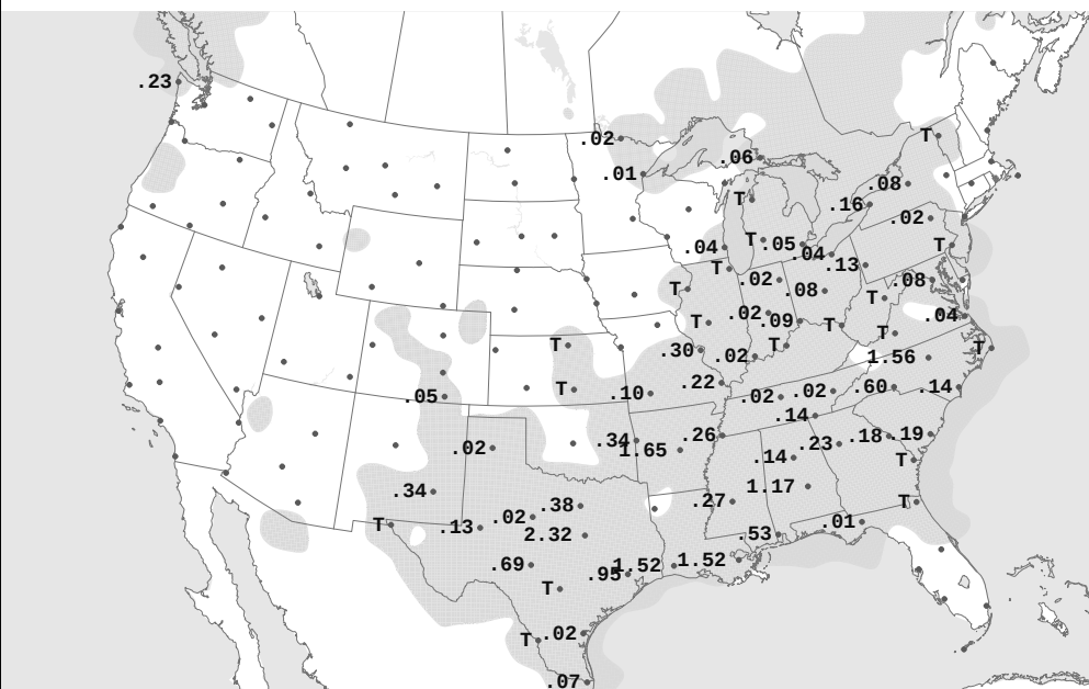
FRI, NOV 25, 2022 24-hour Precipitation Areas and Amounts Ending 7:00 A.M. E.S.T.
