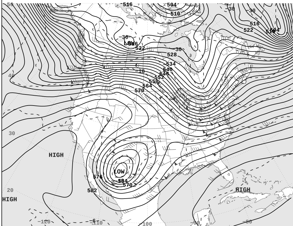
FRI, NOV 25, 2022 500-Millibar Height Contours at 7:00 A.M. E.S.T.
