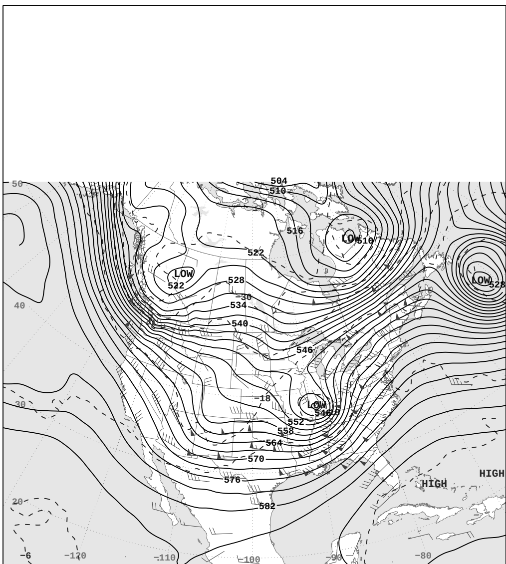
SUN, NOV 27, 2022 500-Millibar Height Contours at 7:00 A.M. E.S.T.
