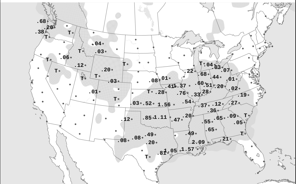
SUN, NOV 27, 2022 24-hour Precipitation Areas and Amounts Ending 7:00 A.M. E.S.T.
