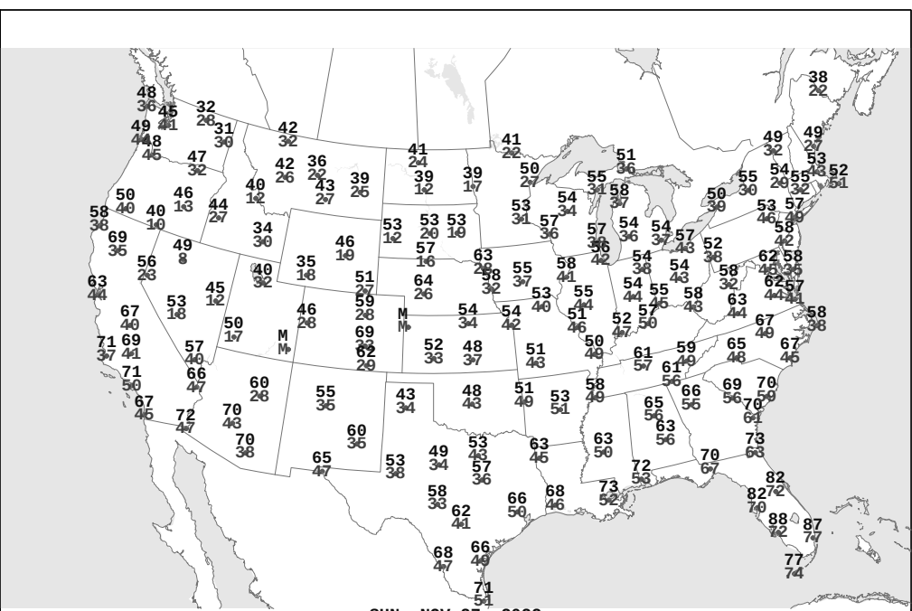
SUN, NOV 27, 2022 Highest and Lowest Temperature
