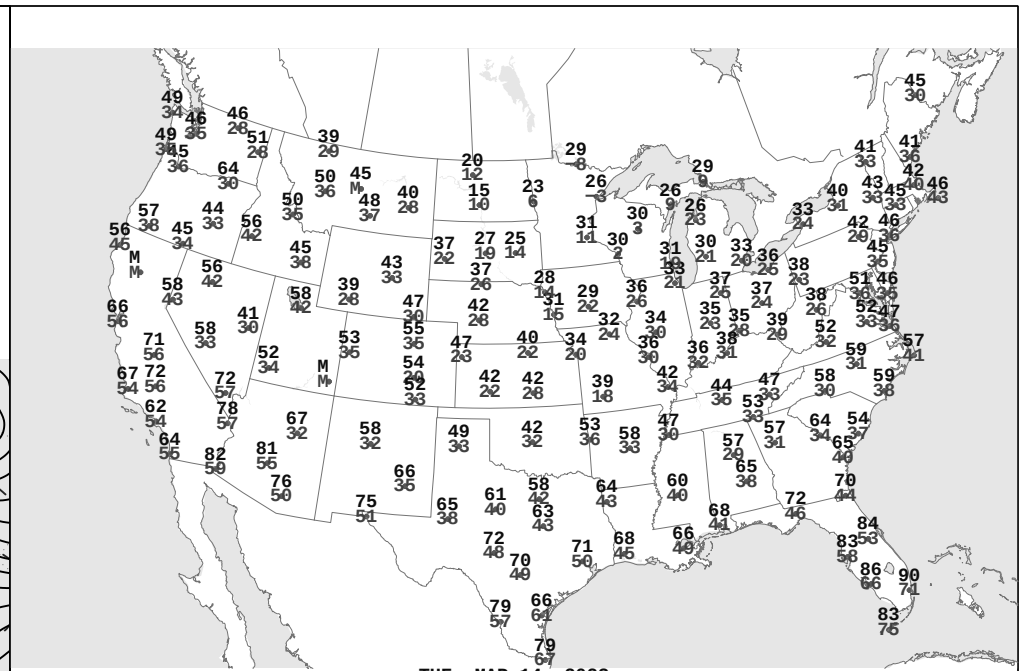
TUE, MAR 14, 2023 Highest and Lowest Temperature
