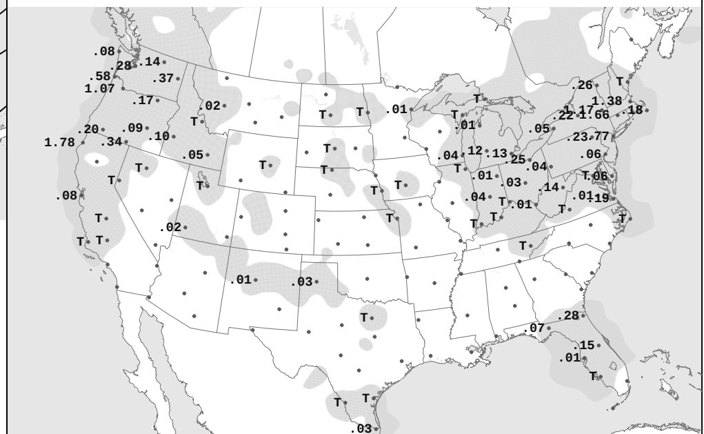
TUE, MAR 14, 2023 24-hour Precipitation Areas and Amounts Ending 7:00 A.M. E.S.T.
