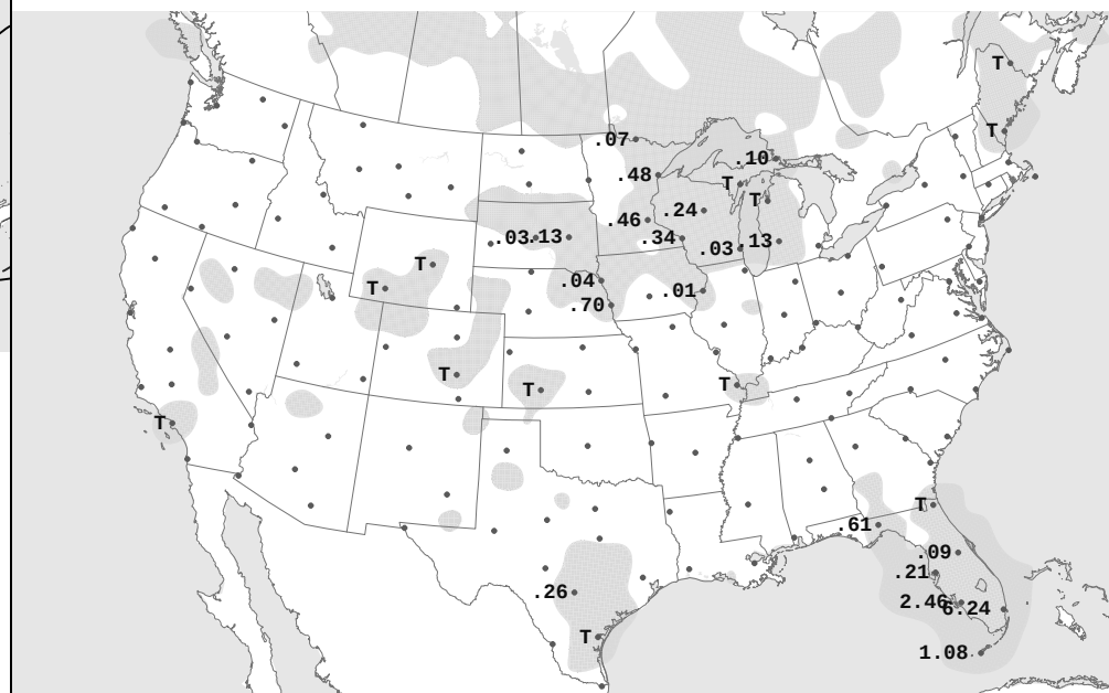
THU, JUN 13, 2024 24-hour Precipitation Areas and Amounts Ending 7:00 A.M. E.S.T.
