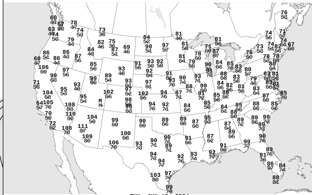
THU, JUN 13, 2024 Highest and Lowest Temperature
