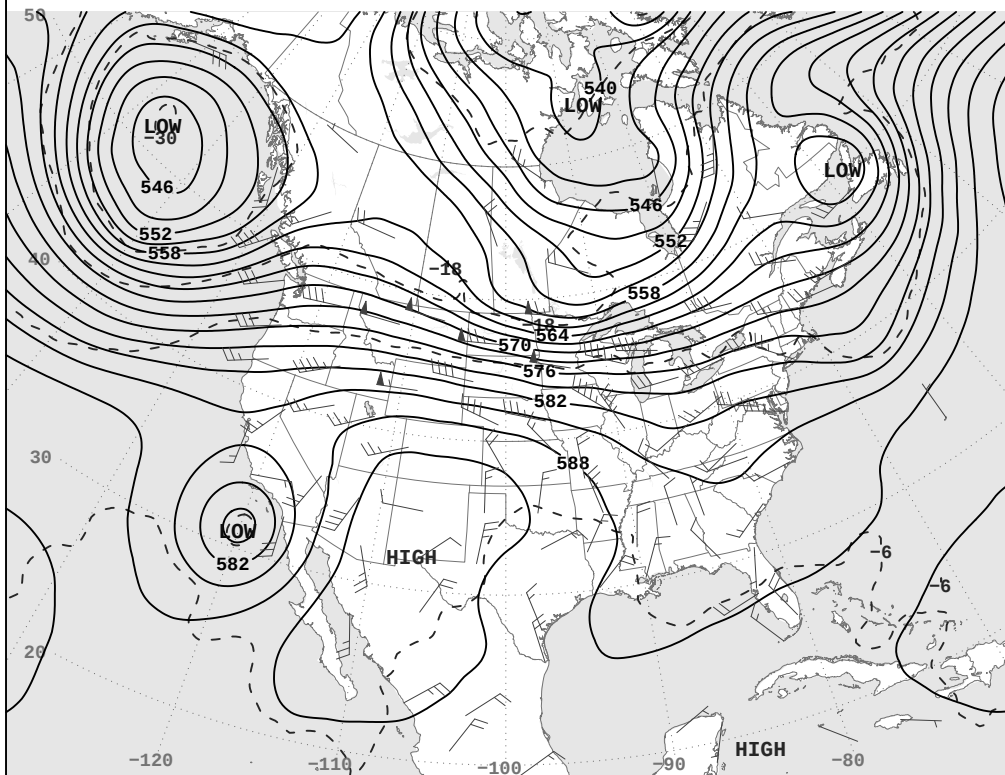
THU, JUN 13, 2024 500-Millibar Height Contours at 7:00 A.M. E.S.T.
