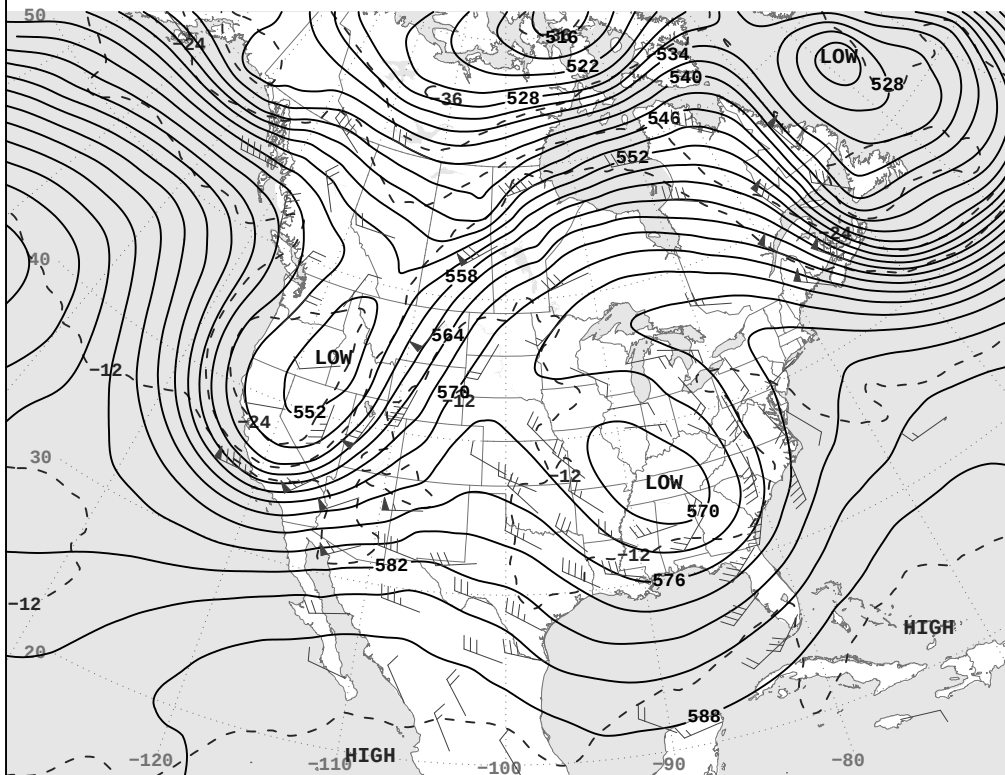
TUE, MAY 13, 2025 500-Millibar Height Contours at 7:00 A.M. E.S.T.
