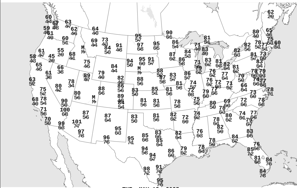
TUE, MAY 13, 2025 Highest and Lowest Temperature
