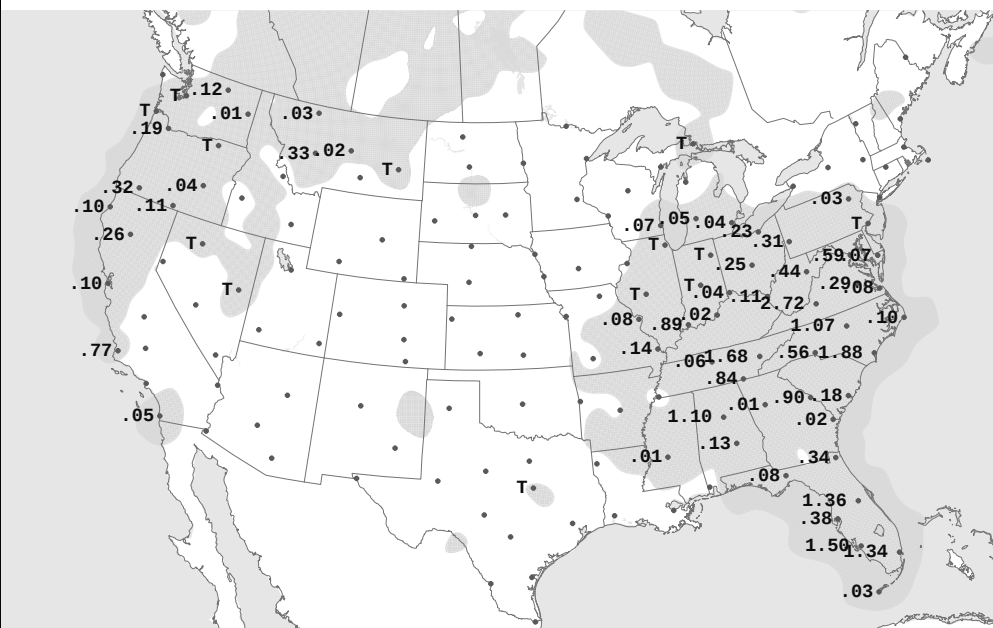
TUE, MAY 13, 2025 24-hour Precipitation Areas and Amounts Ending 7:00 A.M. E.S.T.
