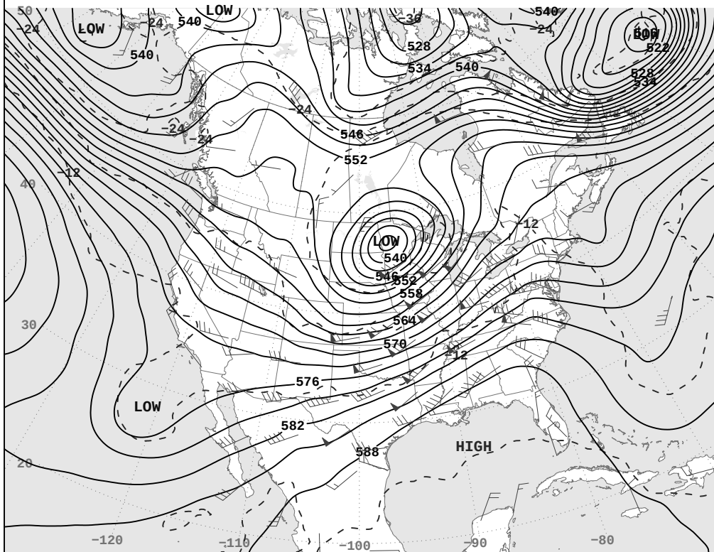
FRI, MAY 16, 2025 500-Millibar Height Contours at 7:00 A.M. E.S.T.
