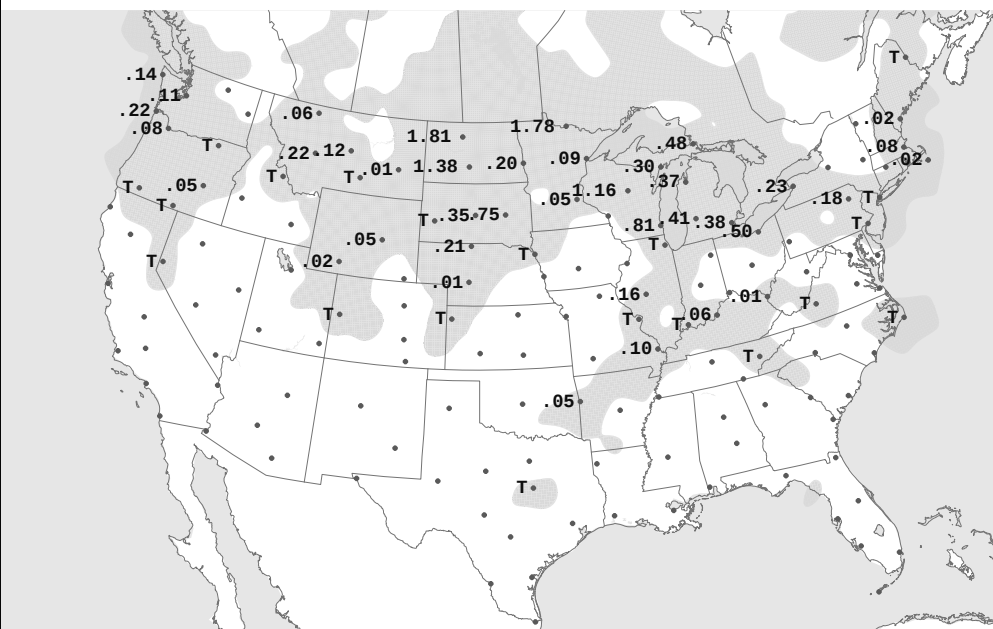
FRI, MAY 16, 2025 24-hour Precipitation Areas and Amounts Ending 7:00 A.M. E.S.T.
