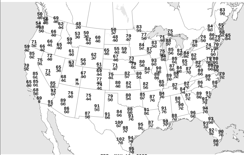
FRI, MAY 16, 2025 Highest and Lowest Temperature
