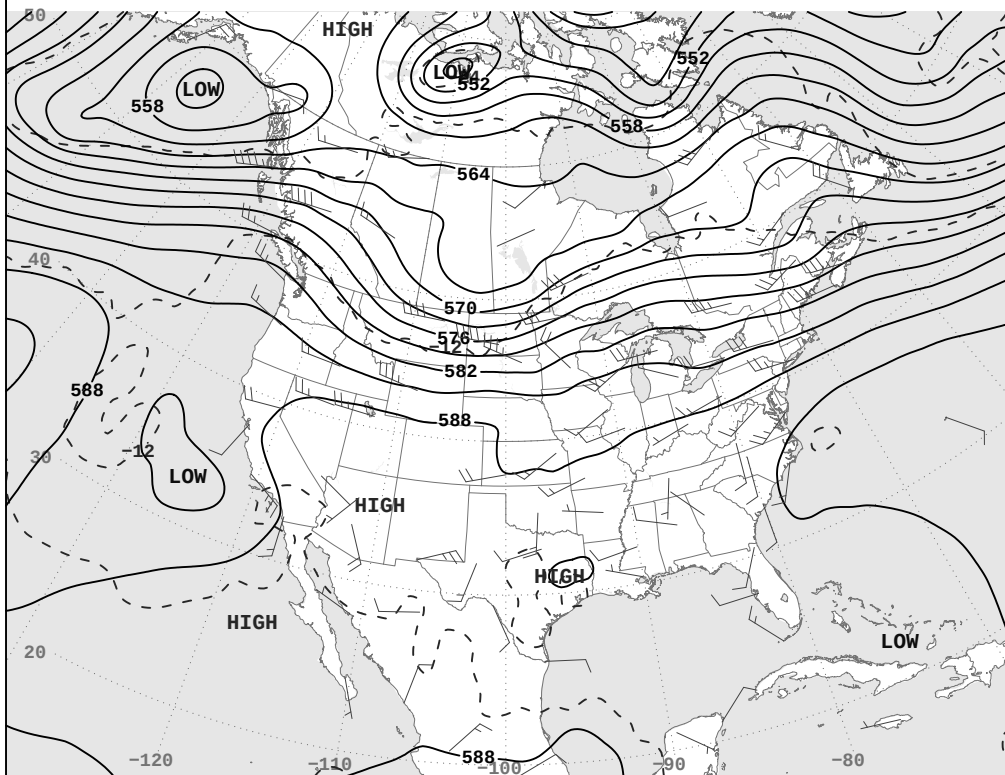
SUN, JUN 29, 2025 500-Millibar Height Contours at 7:00 A.M. E.S.T.
