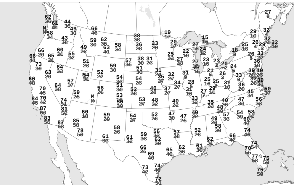
THU, FEB 05, 2026 Highest and Lowest Temperature
