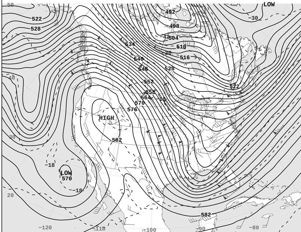
THU, FEB 05, 2026 500-Millibar Height Contours at 7:00 A.M. E.S.T.
