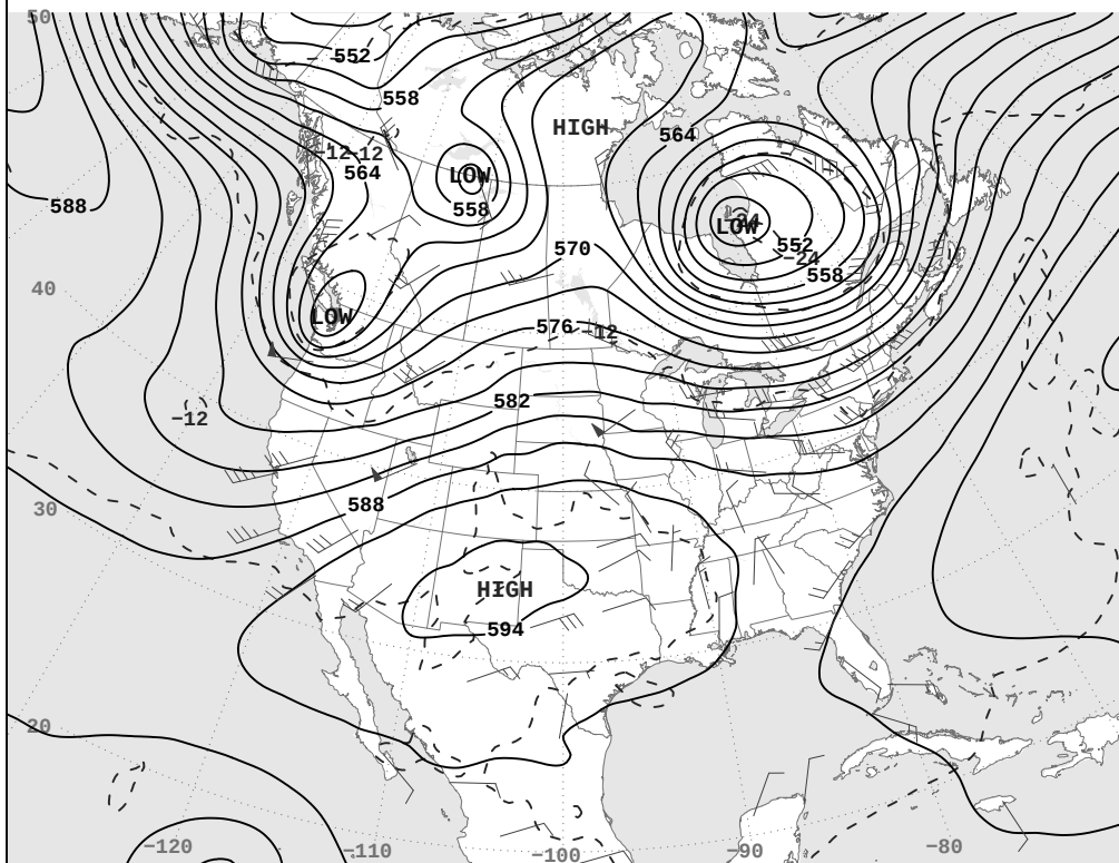
SAT, AUG 29, 2026 500-Millibar Height Contours at 7:00 A.M. E.S.T.
