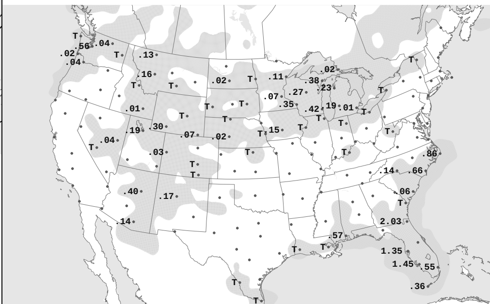
SUN, AUG 30, 2026 24-hour Precipitation Areas and Amounts Ending 7:00 A.M. E.S.T.
