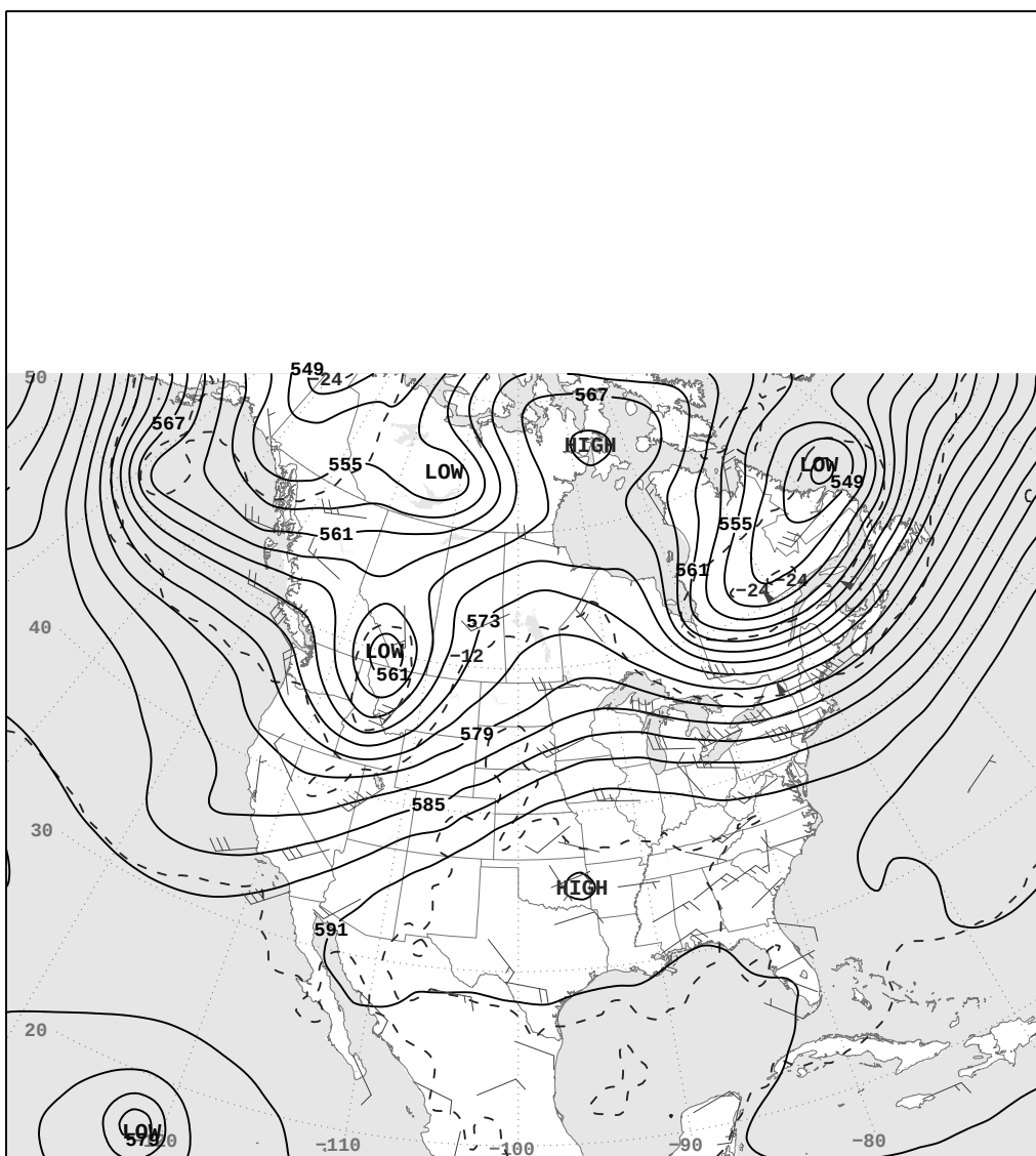
SUN, AUG 30, 2026 500-Millibar Height Contours at 7:00 A.M. E.S.T.
