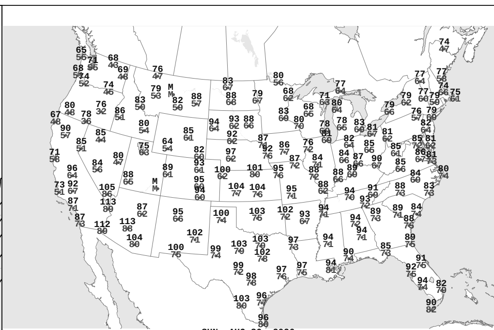
SUN, AUG 30, 2026 Highest and Lowest Temperature
